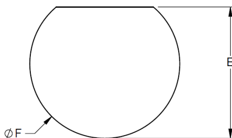
Q38 Jam Nut (RJ) Maximum Panel Thickness: 0.125" (3.18mm)
