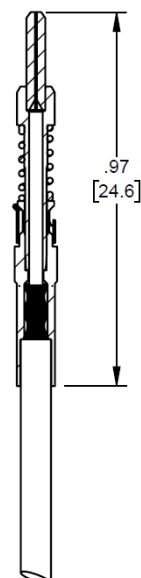
Q38HD-TRM-E2 (Epoxy Cup, 2mm Cable)
