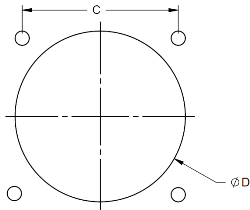
Q38 Internal Flange Mount (RF) Maximum Panel Thickness: 0.125" (3.18mm)
