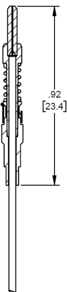
Q38HD-TRM (No Crimp, 900µm Fiber)
