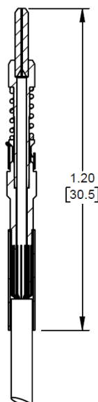
Q38HD-TRM-CM & Q38HD-CMP-2MM (With Crimp, 2mm Cable)
